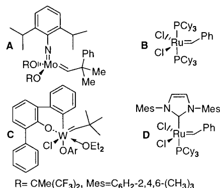
Figure 1. RCM catalysts.
